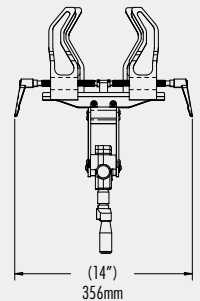
SPIDER 125 with UNIVERSAL CLAMPING
