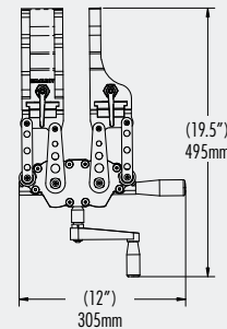
SPIDER 125 with UNIVERSAL CLAMPING
