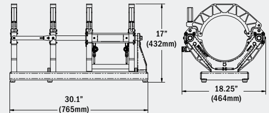
ACROBAT 250 4-JAW CARRIAGE
