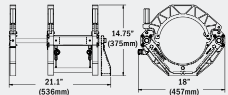
ACROBAT 250 3-JAW CARRIAGE
